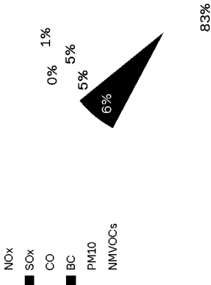
Distribution of air pollutants at sea
